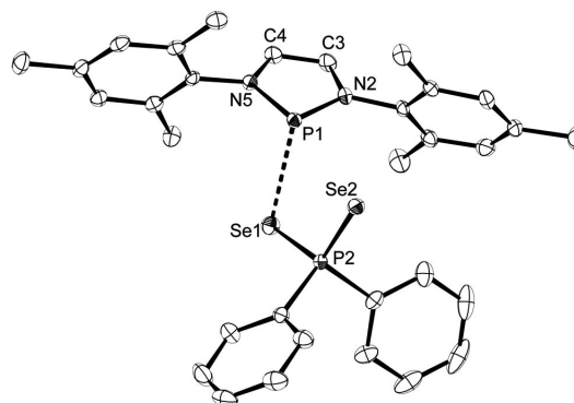
Figure 1. Molecular structure of 2 . Thermal ellipsoids are drawn with 50% probability level, and H atoms have been omitted for clarity. Selected bond lengths [Å] and angles [°]: P1–N2 1.688(2), P1–N5 1.689(2), P1–Se1 2.766(1), P1–Se2 3.391(1), P2–Se1 2.193(1), P2–Se2 2.135(1), N2–C3 1.402(3), C3–C4 1.343(3), C4–N5 1.398(3); N2–P1–N5 88.5(1), N2–P1–Se1 108.3(1), N5–P1–Se1 102.6(1), N2–P1–Se2 104.9(1), N5–P1–Se2 166.6(1), Se1–P1–Se2 72.60(2), P2–Se1–P1 92.76(2), Se2–P2–Se1 116.48(3), P2–Se2–P1 77.99(2).
