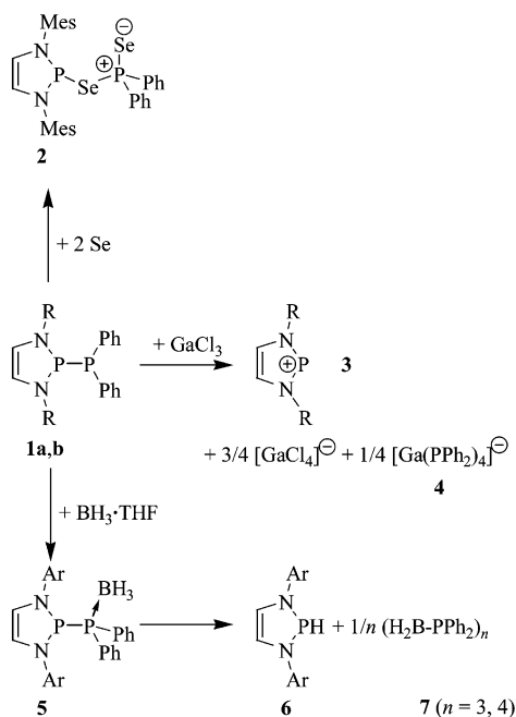
Scheme 2. Reactions of the diphosphanes 1a/b [ 1a : R = Mes (2,4,6-Me 3 C 6 H 2 ); 1b : R = 2,6-Me 2 C 6 H 3 ; 5 , 6 : Ar = 2,6-Me 2 C 6 H 3 ].
